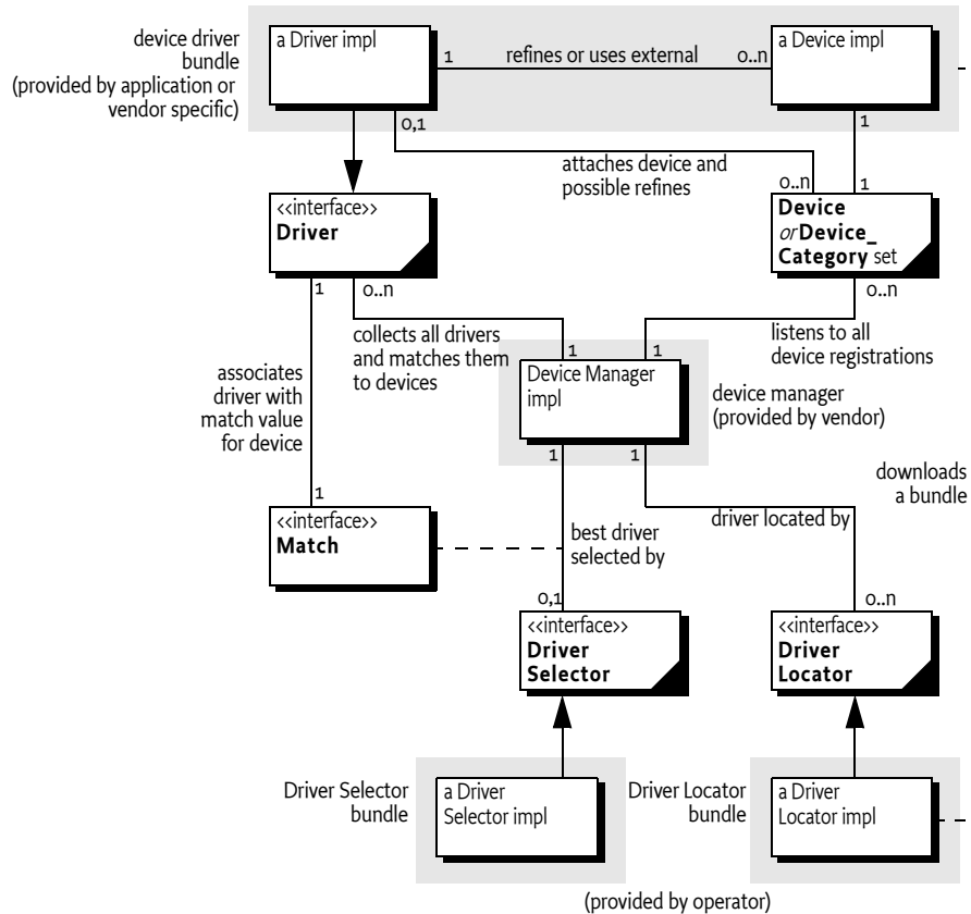
Figure 103.1 Device Access Class Overview
